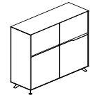
文件柜 EP91 Cabinet W1224*D425*H802 W1224*D425*H1232 W1224*D425*H1552 W1224*D425*H1752
